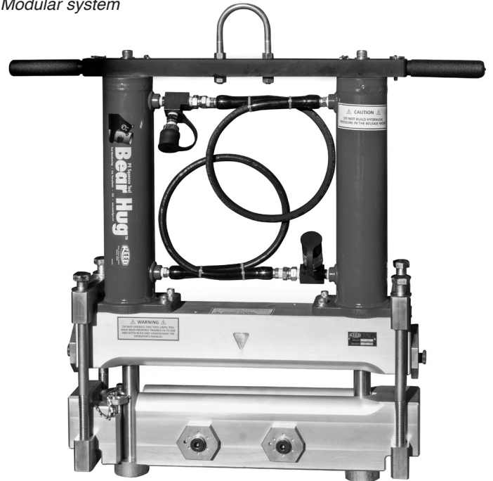
PES8BT Base Tool
